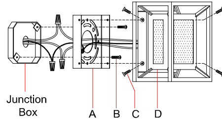
Fig. 1 Wall Sconce
