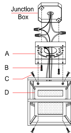
Fig. 2 Ceiling Mount
